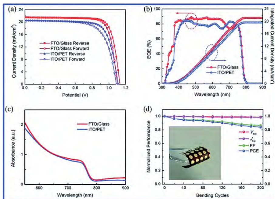
Fig. 20 The best-performing devices based on PEALD \text{SnO}_2 coated FTO/glass and ITO/PET substrates: (a) J-V curves under reverse and forward voltage scans. (b) EQE spectra and their corresponding integrated photocurrents. (c) Absorption spectra of perovskite films. (d) Normalized performance parameters of a flexible PVSC versus bending cycles. Photograph of a flexible device after the bending test (inset), 300 presented with permission and copyright.
